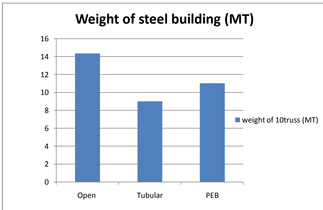
Fig. 1. Weight comparison between sections
