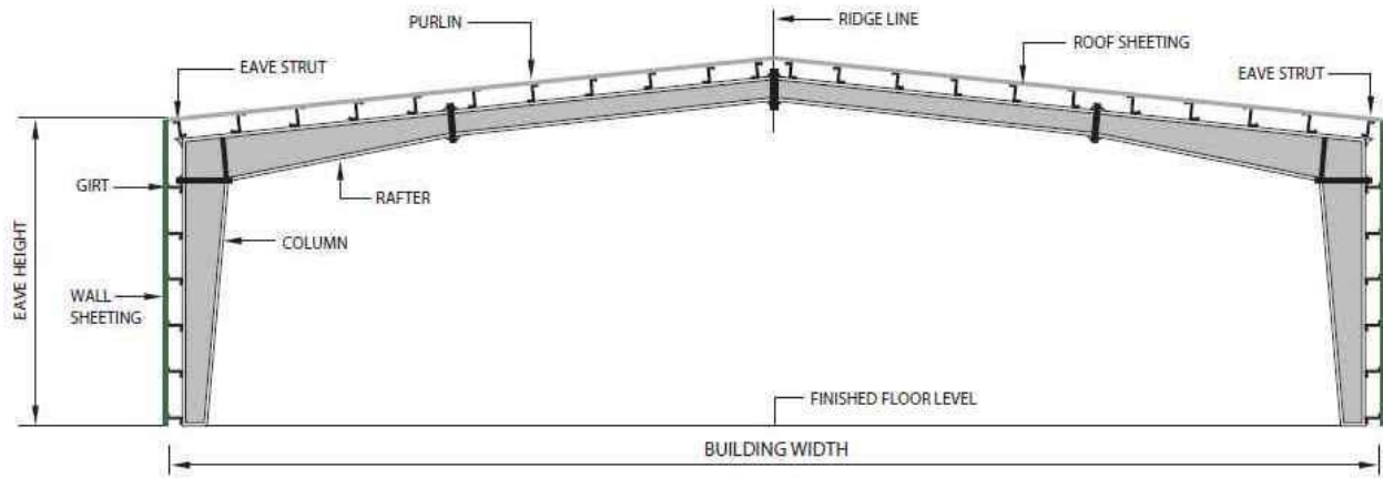
Fig.1 Typical Cross section of PEB
